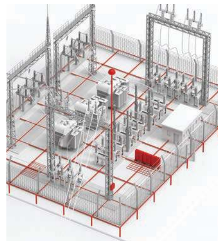
nVent ERICO System 3000 Collection Volume Method (Active System)
