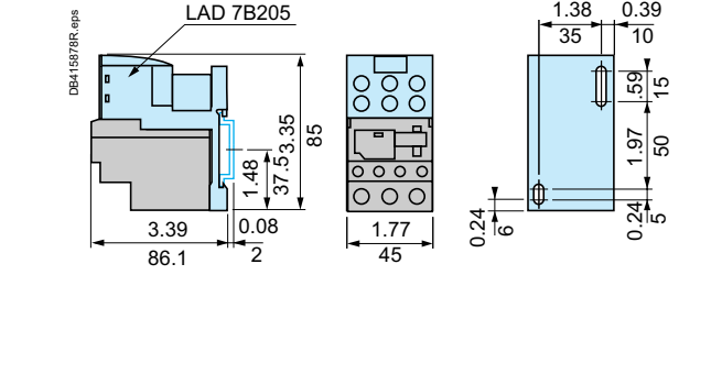
LRD04L-32L Independent mounting on 1.97 in. (50 mm) centers or on rail AM1DP200 or DE200
