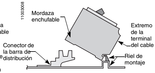
Figura 6: Homeline Tandem Circuit Breaker
