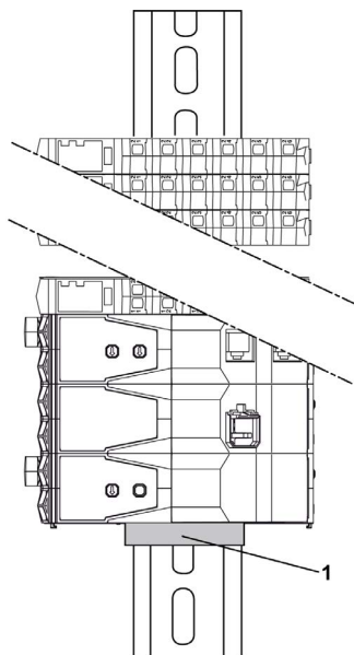
1 End bracket
