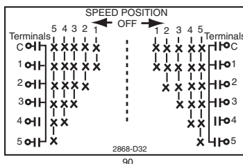
Single Speed Contact Symbols
