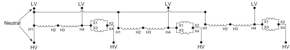
Wiring Diagram 9
