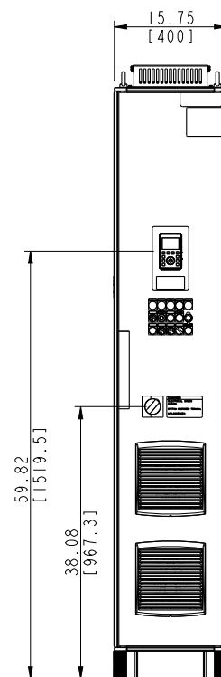
FRONT VIEW
