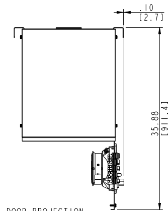
DOOR PROJECTION
