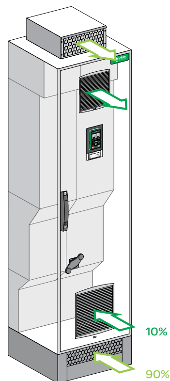
Cooling concept
