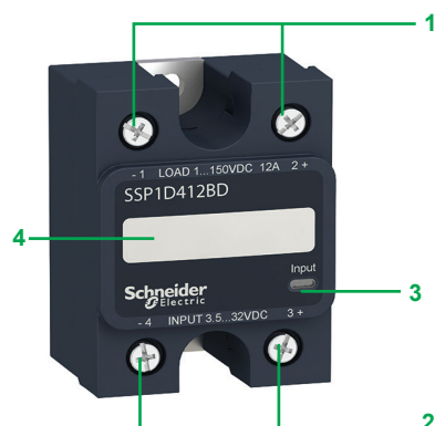
SSP1 single-phase panel mount relays
