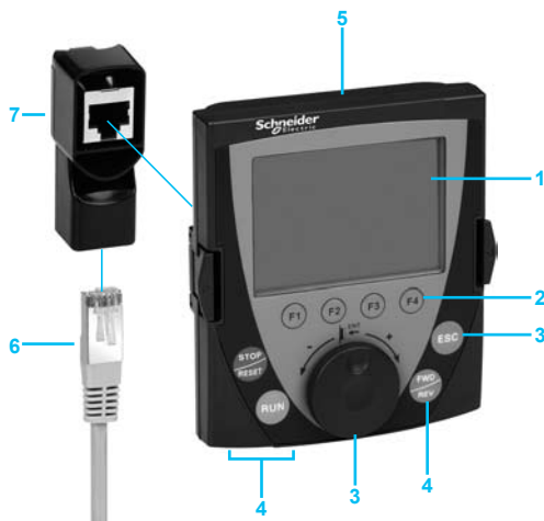
Graphic display terminal + female/female RJ45 adaptor + remote cable
