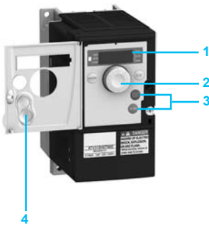
ATV 312H075M2 front panel door open
