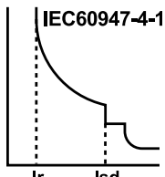
MicroLogic 2.2M and 2.3M Trip Units
