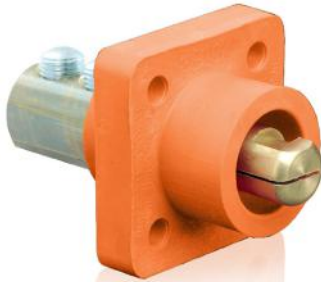
Male Panel Mount Receptacle - Double Set Screw (18R23-UO Shown)
