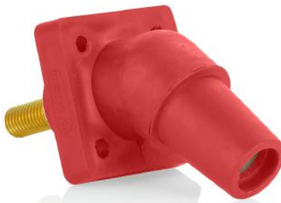
Female - 1.125"L Threaded Stud Termination (16R30-1UR Shown)
