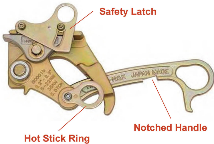
HOT LINE POWER GRIPS™ - with SPRING-LOADED SAFETY LATCH, HOT STICK RING, & NOTCHED HANDLE
