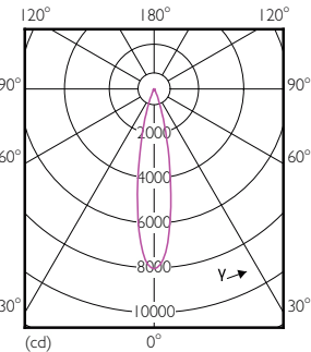
Light Distribution Diagram - 17PAR38/EXPERTCOLOR/F25/940/DIM
