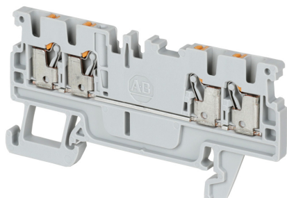
Terminal Blocks—Dimensions (W x H x L): 3.5 x 33.5 x 67.5 mm
