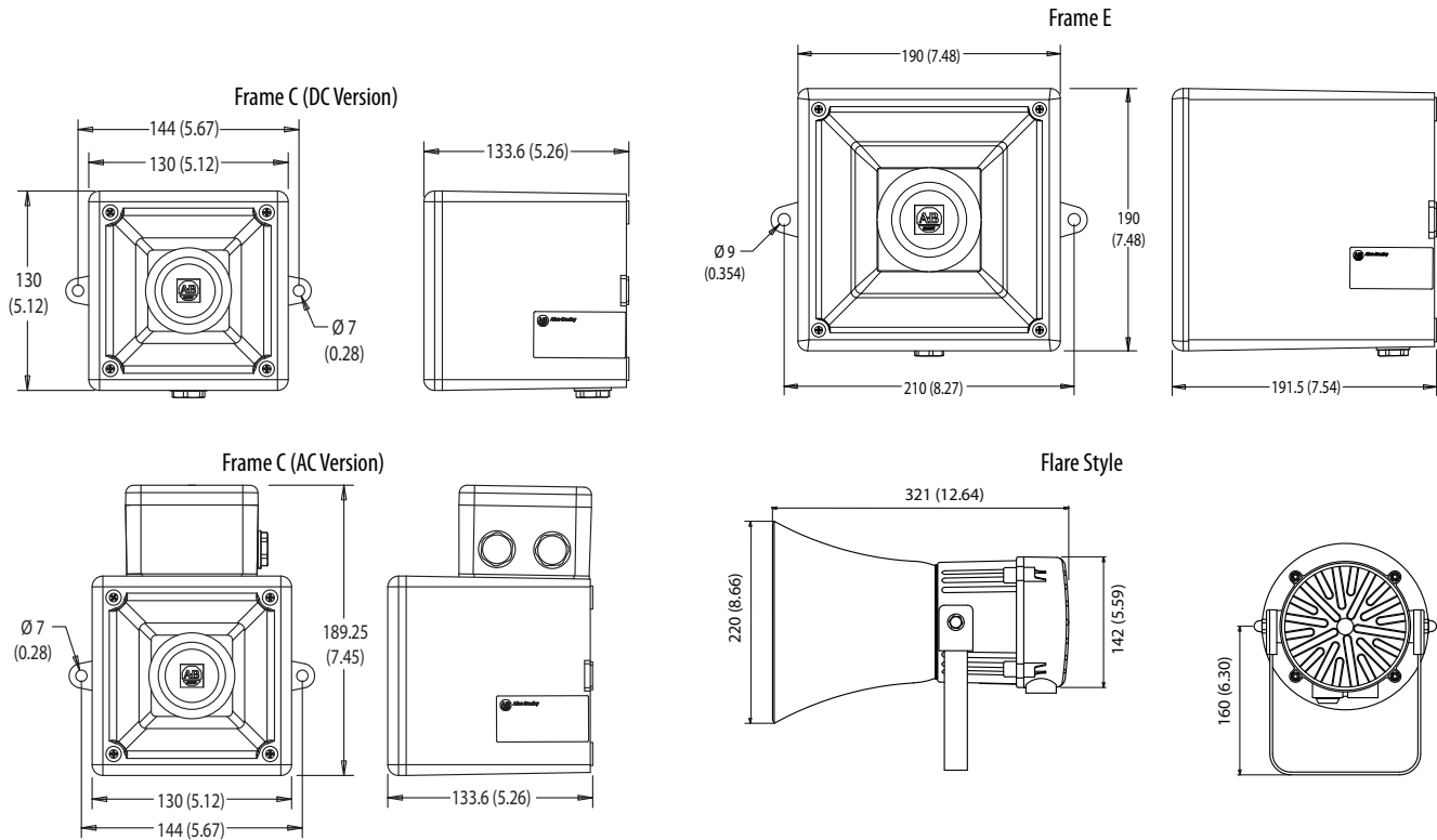
Figure 3 - Recordable Horns
