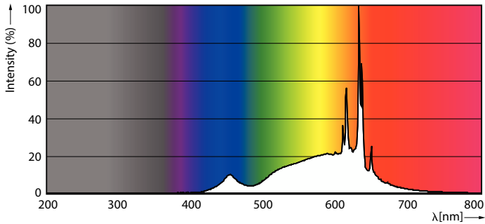
Spectral Power Distribution Colour - 8.8A19/COR/927/FR/P/E26/DIM/T20 6/1CT
