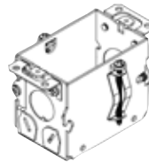
SBG523 MC Clamp for old work with locking grips
