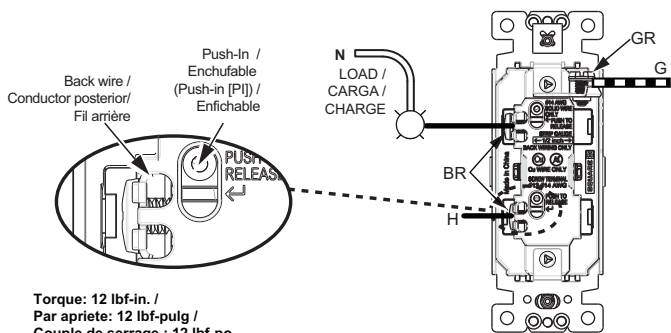
FIG 1: Wiring Diagram for SQR14101XX / SQR14201XX / SQR14106XX Diagrama de cableado / Schéma de câblage
