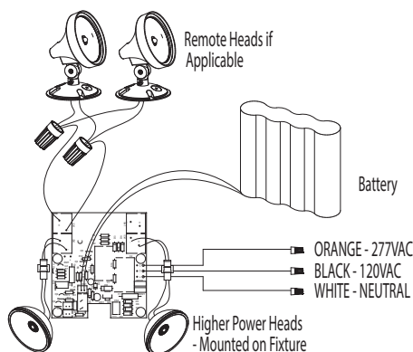
SEL with Remote Capacity and Higher Power Heads
