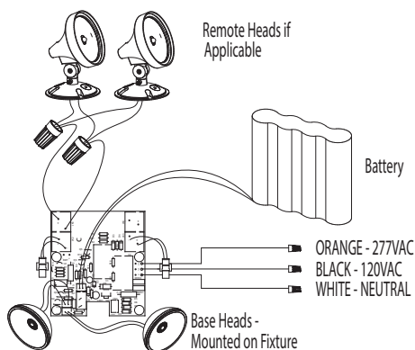
SEL with Remote Capacity and Base Heads
