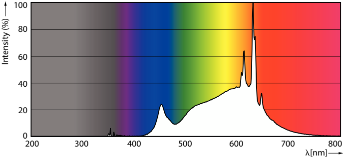
Spectral Power Distribution Colour - 8.5PAR30S/LED/930/F25/DIM/GULW/T20 6/1FB
