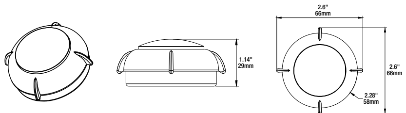
Zhaga Bluetooth Sensor Side View
