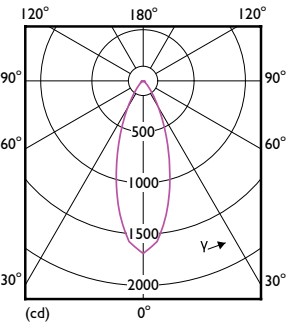
Light Distribution Diagram - 8.5PAR30L/LED/930/F40/DIM/GULW/T20 6/1FB
