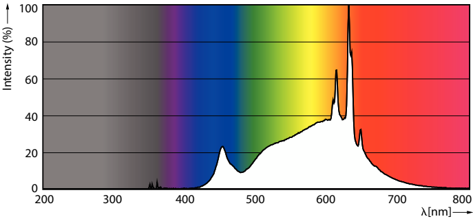
Spectral Power Distribution Colour - 8.5PAR30L/LED/930/F40/DIM/GULW/T20 6/1FB
