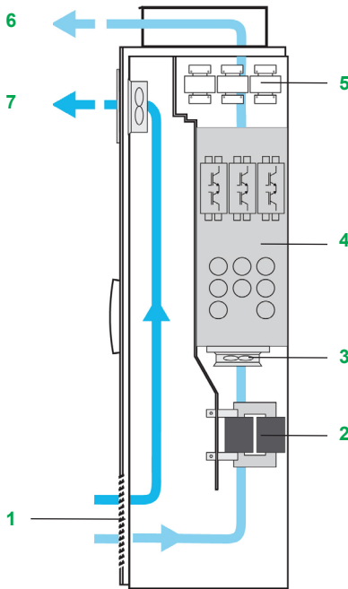
IP23 enclosure
