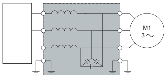
Sinus filter
