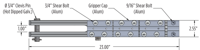
Bolted Nut Clevis (BN) Hot Dip Galvanized (Optional) Stainless Steel Also Available
