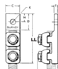
Type QQA
