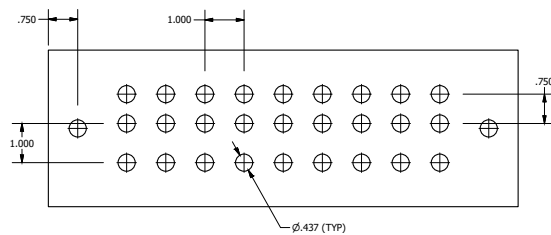
Pattern J
