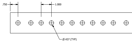
Pattern H
