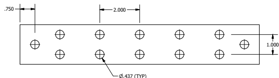
Pattern B
