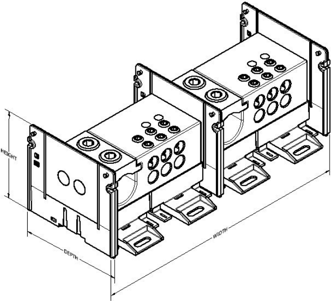
Double-Wide Lay-In Two Pole BDBLCS13LK2DW shown
