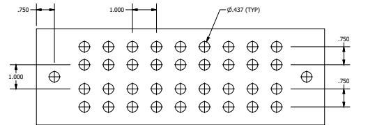
Pattern W
