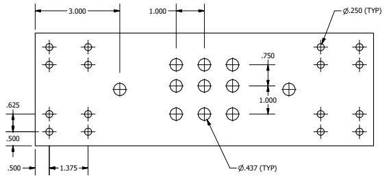
Pattern V
