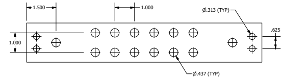
Pattern X
