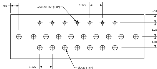
Pattern F
