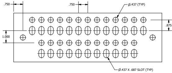
Pattern M
