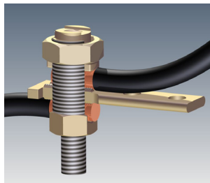
Splice Connection
