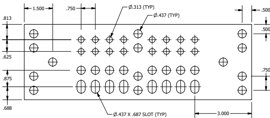
Pattern Q
