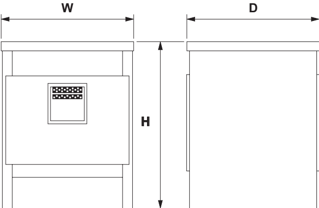
Style 1 - Ventilated
