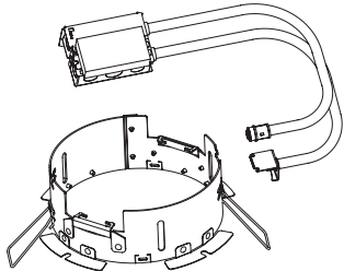
HC6 LED Retrofit Rough-in Section
