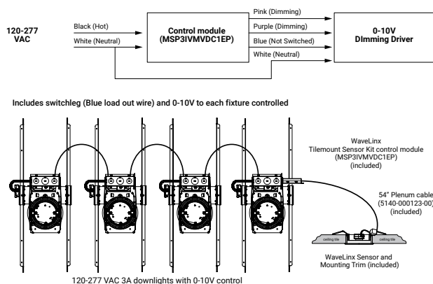
WaveLinx WTA Tilemount Wiring Diagram
