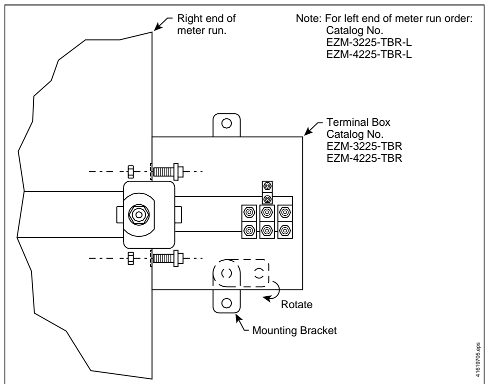
Figure 1: Mounting the Meter/Breaker
