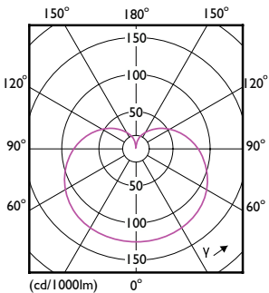
Light Distribution Diagram - 16.6A19/LED/950/FR/P/E26/ND/T20 6/1FB
