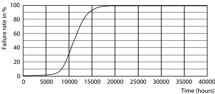
Life Expectancy Diagram - 16.6A19/LED/950/FR/P/E26/ND/T20 6/1FB
