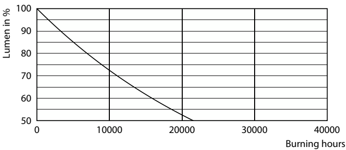
Lumen Maintenance Diagram - 16.6A19/LED/950/FR/P/E26/ND/T20 6/1FB
