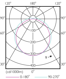
Light Distribution Diagram - 12PL-C/T/COR/32H-840/IF14/P/4P/DIM 10/1
