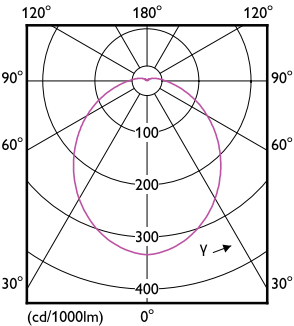
Light Distribution Diagram - 5R20/PER/927/P/E26/DIM 6/1FB T20
