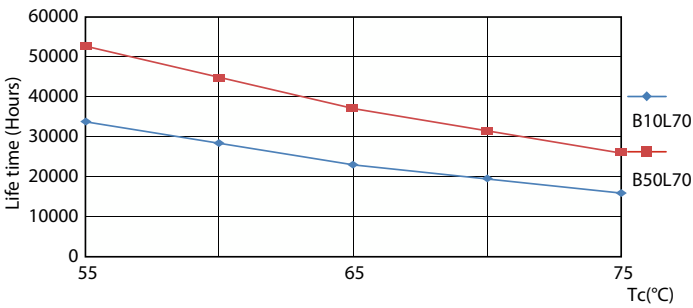
Life Expectancy Diagram - 42T8HO/COR/96-840/MF54/G/R17d 10/1
