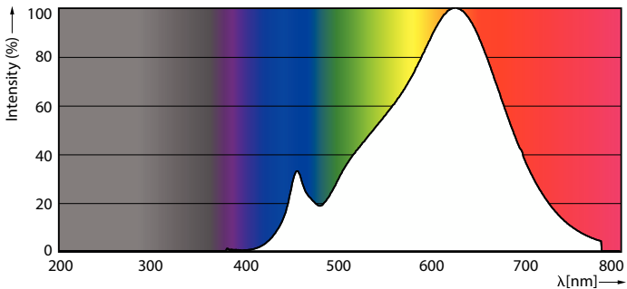
Spectral Power Distribution Colour - 7.8MR16/PER/927/F35/Dim/EC/12V 10/1FB
