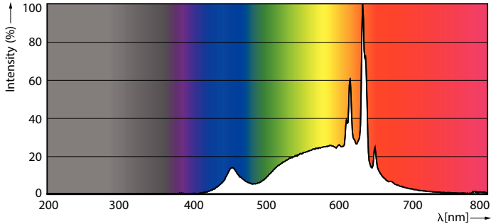
Spectral Power Distribution Colour - 8.8A19/LED/927/FR/P/E26/ND/T20 6/1FB
