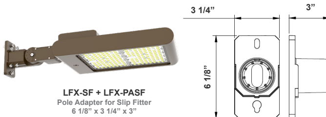
LFX-TR-A U Bracket 13 3/8" x 10 1/8"
