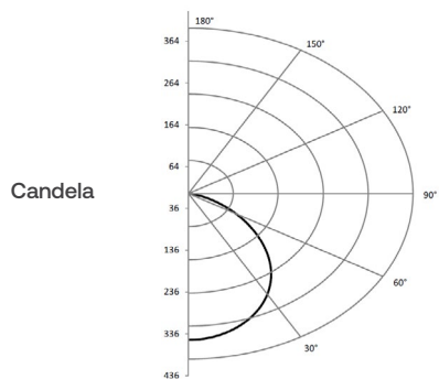
LED8DRS4/9SC Polar Plot
