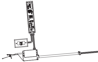
PR6 LED Retrofit REM Rough-in Section
