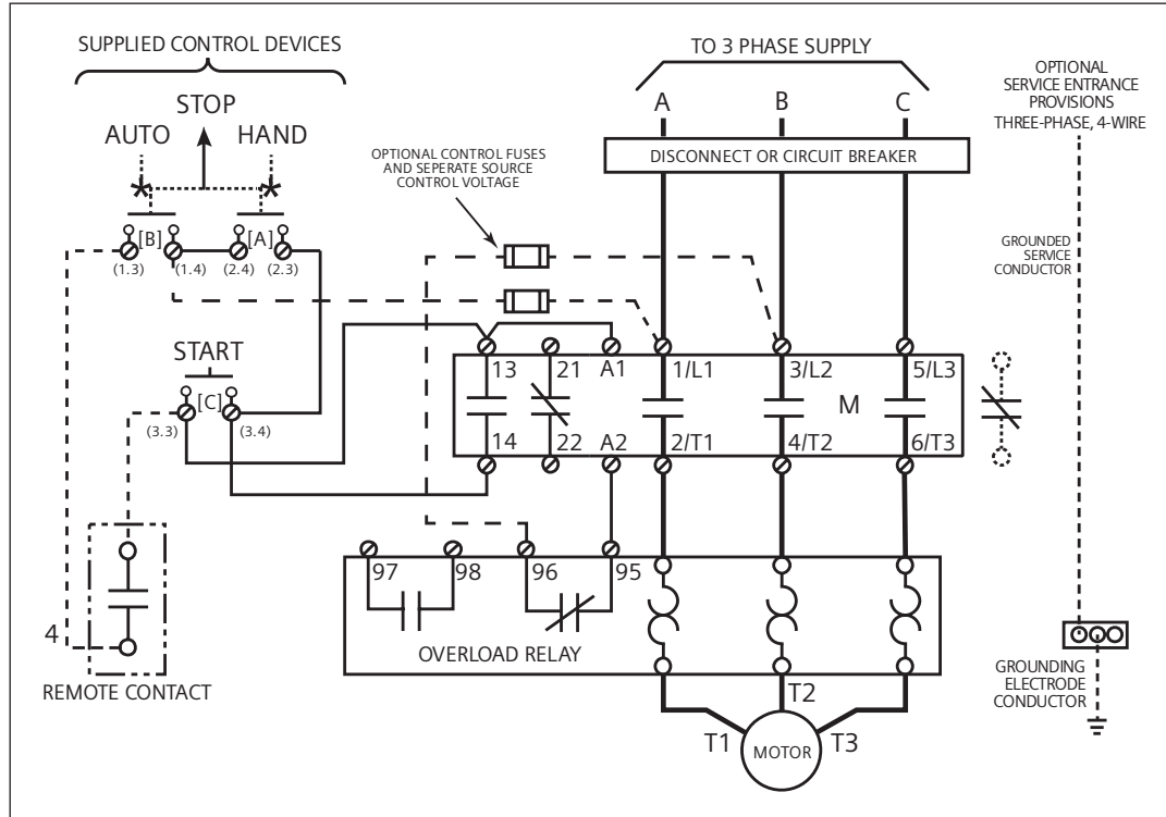
3RE48 Pump Panel
