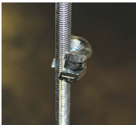
Rod Lock Height-Adjustable Strut Nut CRLSL37EG
