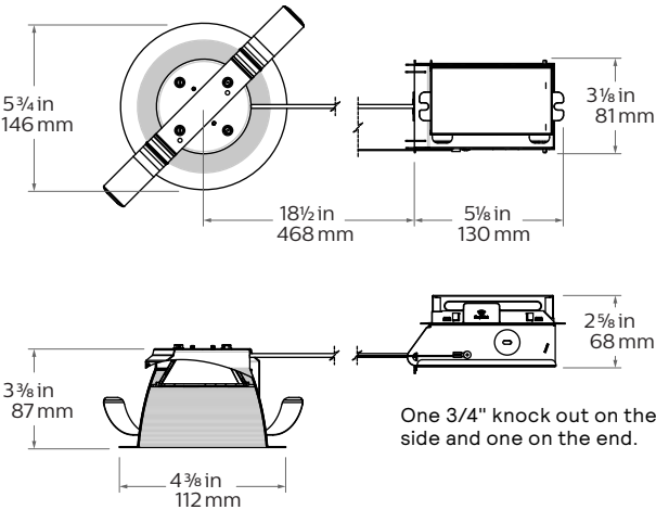
Flex Install (F)
