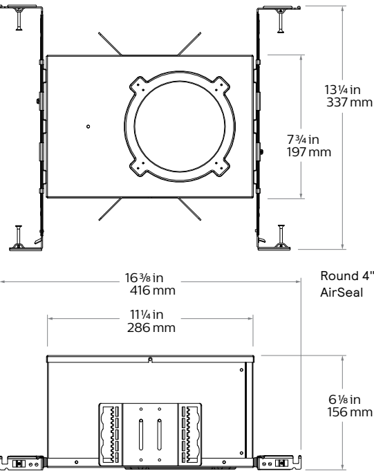
AirSeal (A) / Chicago plenum (LC)
