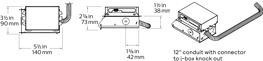
LCEM6 Flex install (F) engine only
