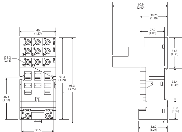
Figure 62 - Cat. No. 700-HN153
