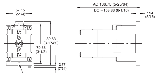
Figure 116 - 6- and 8-pole 700S-P Relay
