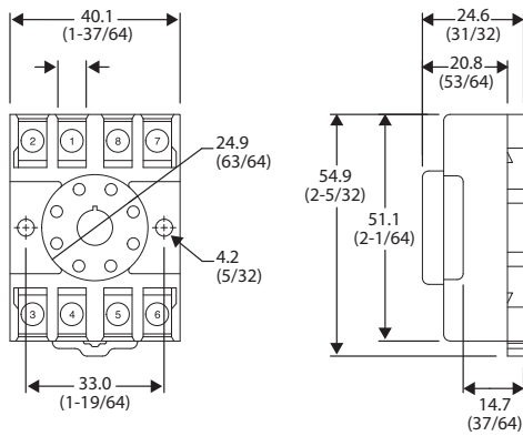
Figure 72 - Cat. No. 700-HN125
