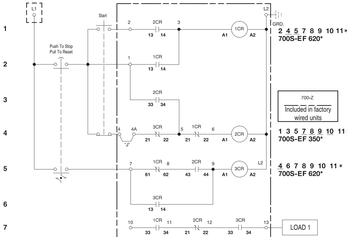
Figure 149 - 700S-EF Circuit
