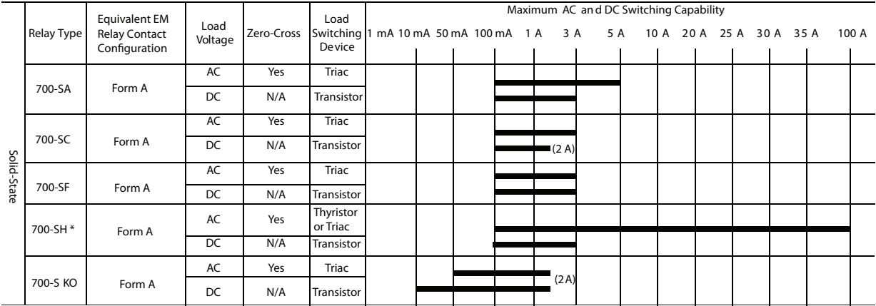
Figure 154 - Solid-state Relay Switching Capacity
