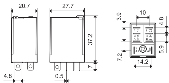
Figure 22 - Cat. No. 700-HF Relay (DPDT)
