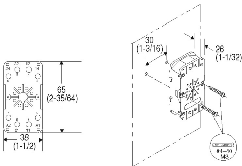
Cat. No. 700-HN100 Wire Size: 2x2.5 mm
