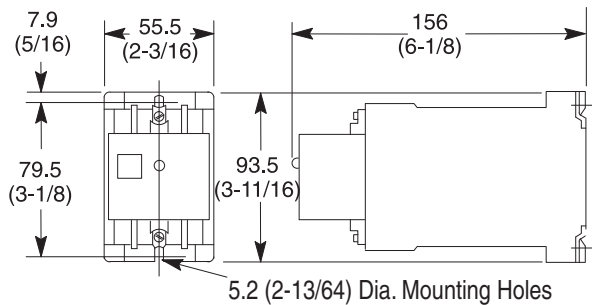
Figure 134 - 700-RTC Relays
