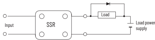
Figure 170 - DC Inductive Load Wiring
