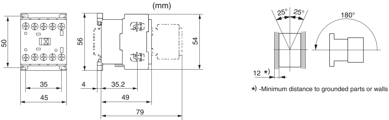
Figure 153 - 700-K Control Relay and Mounting Position
