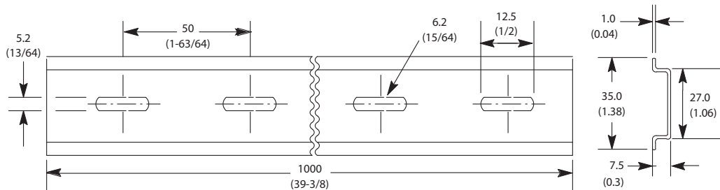
Figure 132 - Cat. No. 199-DR1 DIN Mounting Rail, Series B
