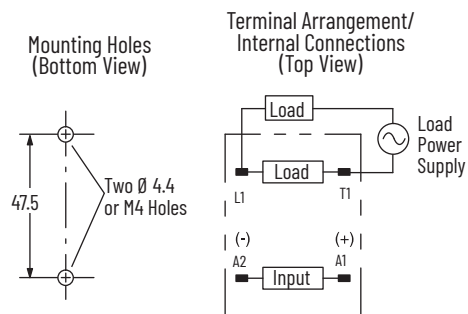
Figure 184 - Mounting Considerations
