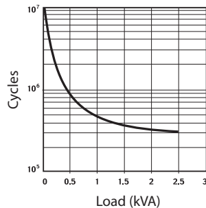
Figure 1 - 700-HA Relay Performance Graphs
