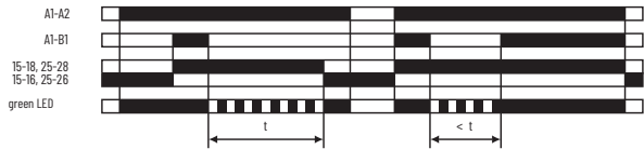
(F) Flasher [Repeat Cycle Starting with Pulse]
