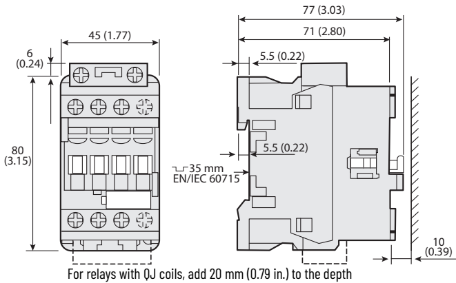
Figure 144 - 700-EF Relays with Standard Coils and Front-mounted Auxiliary Contact
