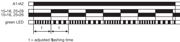
(G) Flasher, Starting with OFF
