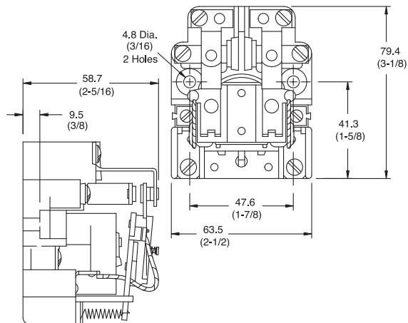
Figure 66 - 700-HG Relay
