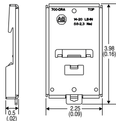
Figure 131 - Cat. No. 700-DRA DIN Rail Adapter
