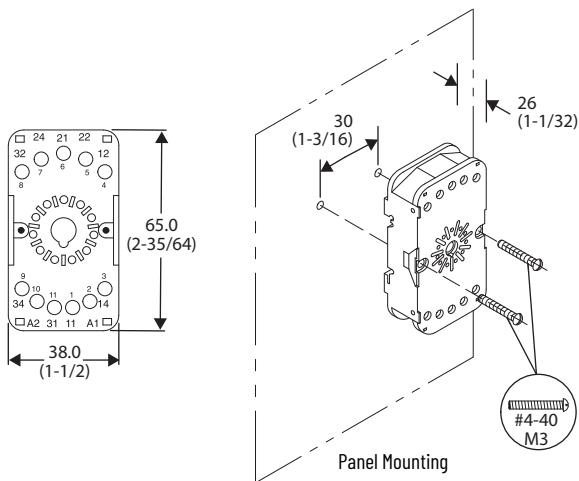
Figure 5 - Cat. No. 700-HN101
