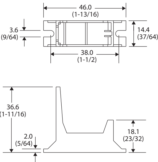
Figure 39 - Cat. No. 700-HN227
