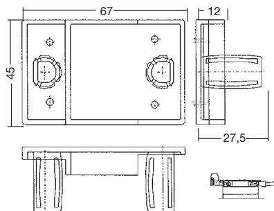
Figure 191 - Cat. No. 700-SHCOV
