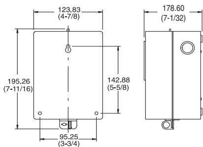
Figure 123 - Drawing No. 4
