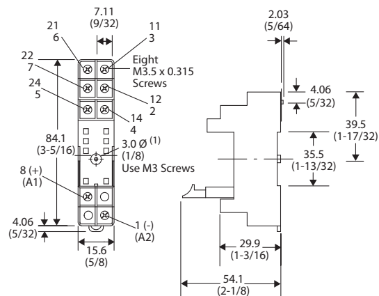
Figure 89 - Cat No. 700-HN122
