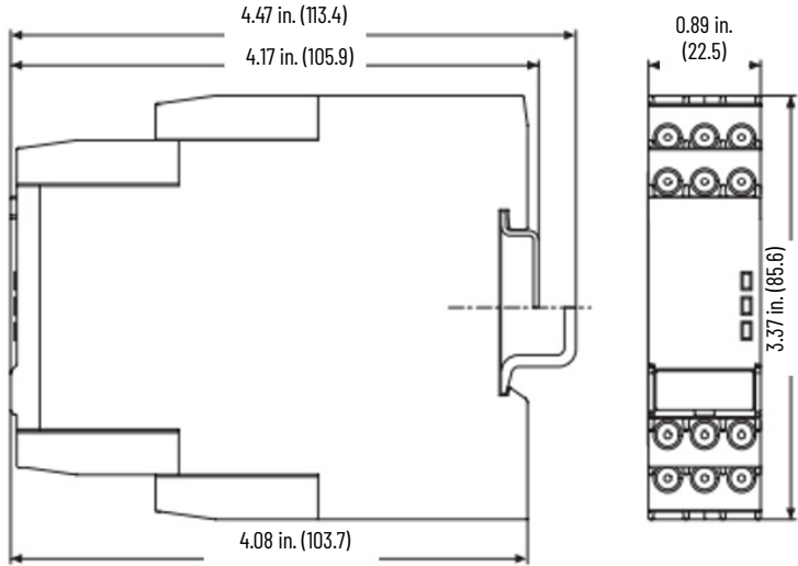
Figure 76 - Cat. No. 700-FS
