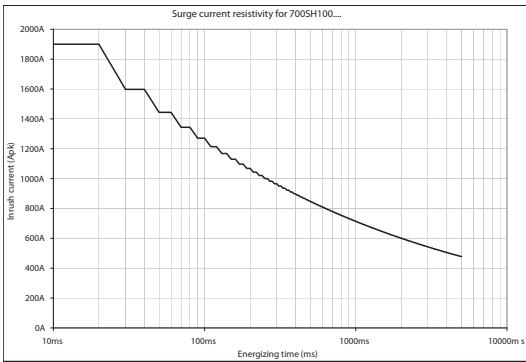
Figure 174 - Surge Current Resistivity Curves, 100 A Devices
