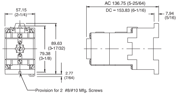
Figure 109 - 700-P Relay, Up to 12 poles with -PB and -PC adder decks
