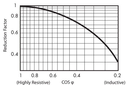
Figure 20 - Load Reduction factor Versus \cos \phi
