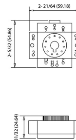
Cat. No. 700-HN126 Wire Size: 2x2.5 mm
