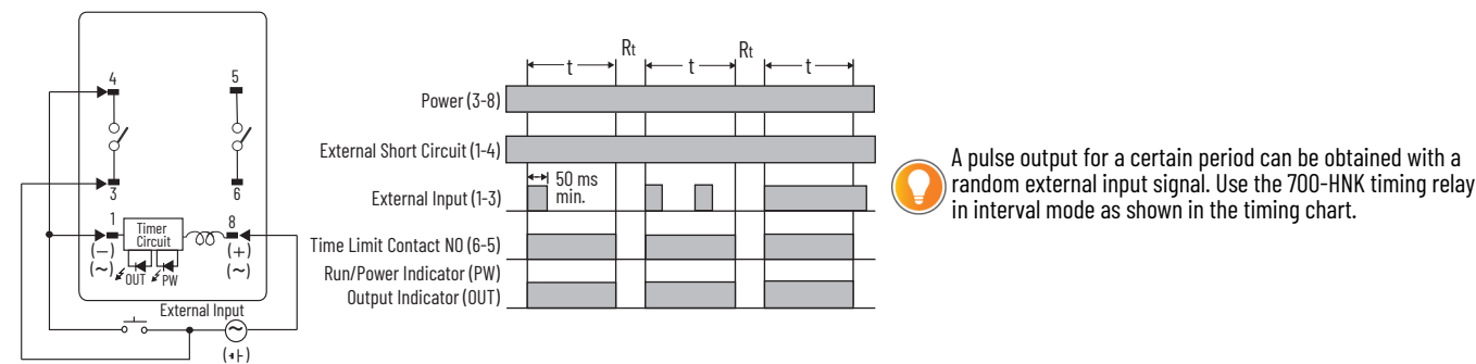
Figure 85 - Wiring
