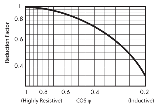
Figure 13 - Load Reduction factor Versus \cos \phi
