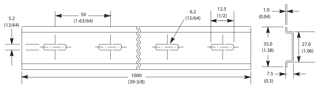
Figure 28 - Cat. No. 199-DR1 DIN Mounting Rail, Series B
