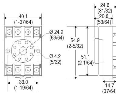
Cat. No. 700-HN125 Wire Size: 2x2.5 mm
