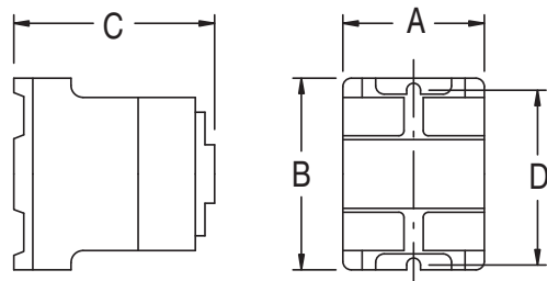
Figure 127 - 700-R400...
