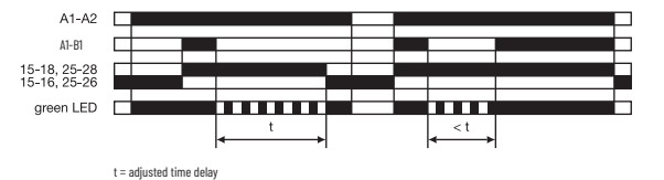
(C) ON-delay and OFF-delay, Symmetrical
