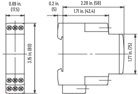
Figure 75 - Cat. No. 700-FE with 2 C/O Contacts
