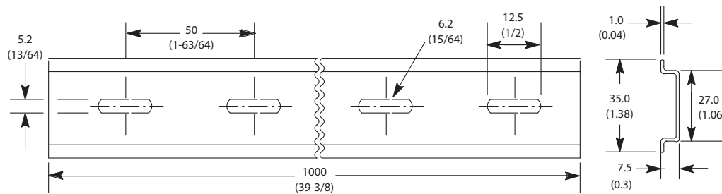
Figure 56 - Cat. No. 199-DR1 DIN Mounting Rail, Series B
