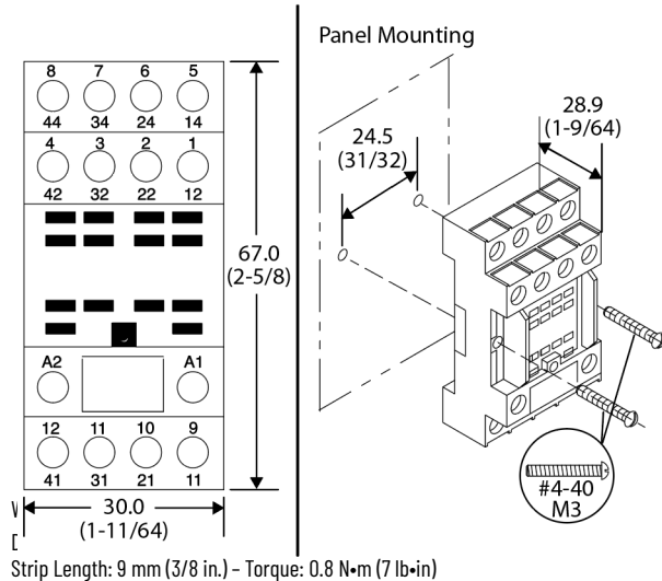
Figure 82 - Cat. No. 700-HN103
