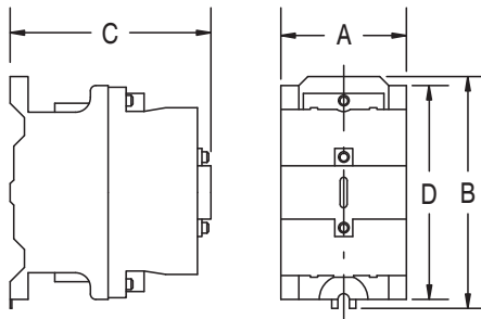
Figure 121 - Drawing No. 2
