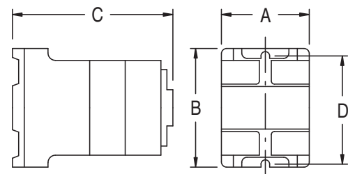
Figure 129 - Type 1 Enclosure
