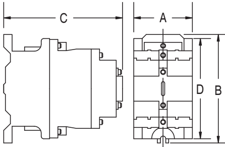
Figure 122 - Drawing No. 3
