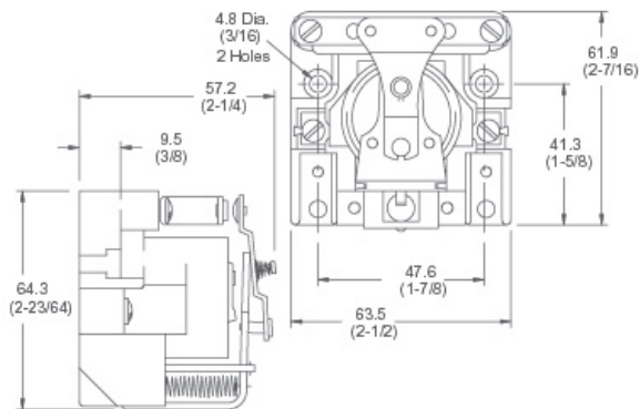
Figure 66 - 700-HG Relay
