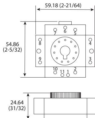
Figure 73 - Cat. No. 700-HN126
