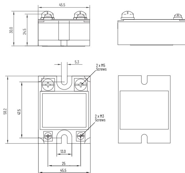
Figure 185 - Cat. No. 700-SH5F...
