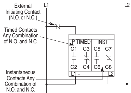
Figure 133 - Typical Wiring Diagram - 700-RTC Relays
