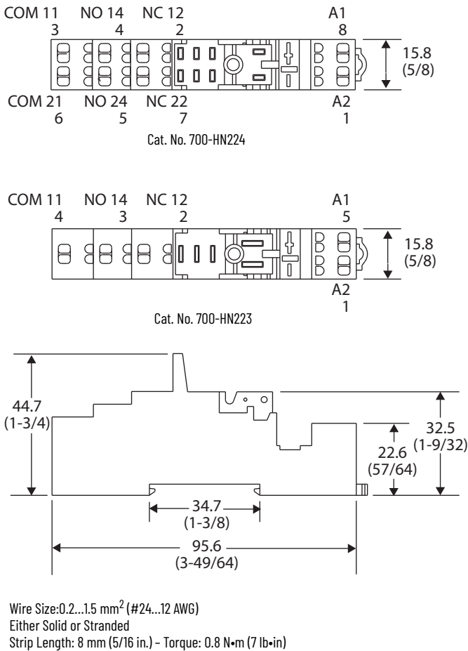
Figure 37 - Cat. No. 700-HN223, -HN224
