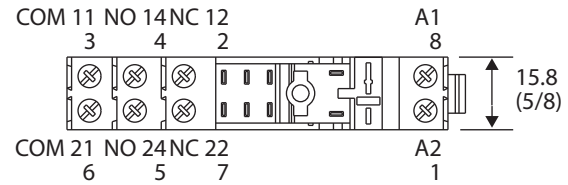
Figure 36 - Cat. No. 700-HN221, -HN222
