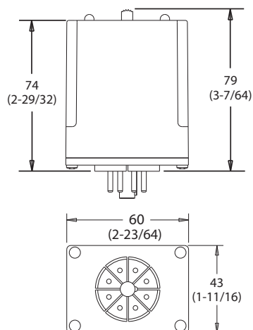
Figure 69 - 700-HTA Relay
