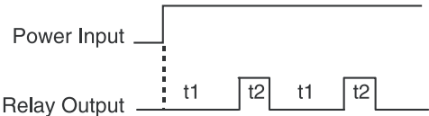
Figure 98 - Timing Diagram- 700-HV Relays
