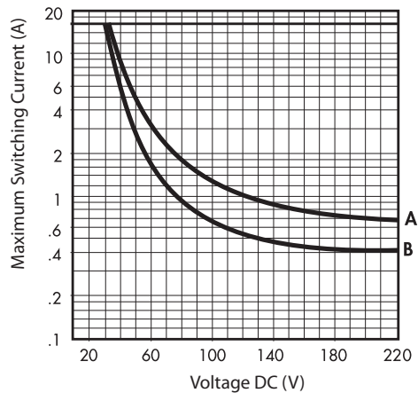
Figure 12 - Breaking capacity for DC-1 load at 600 cycles/hour
