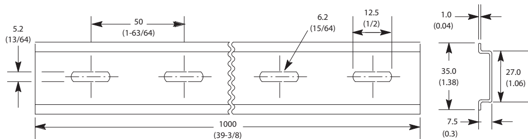
Figure 3 - Cat. No. 199-DR1 DIN Mounting Rail, Series B
