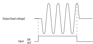
Figure 181 - Zero Cross Function
