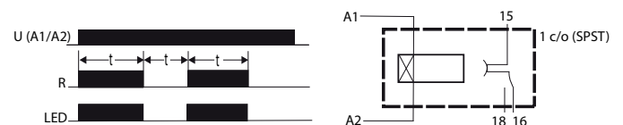
Figure 54 - Flasher
