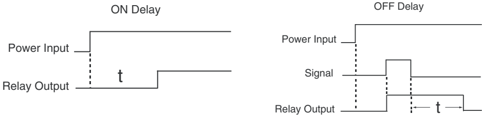
Figure 96 - Timing Diagrams for 700-HT Relays
