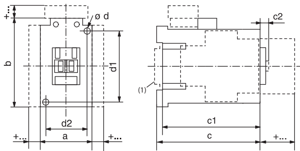
Figure 136 - Mounting Position
