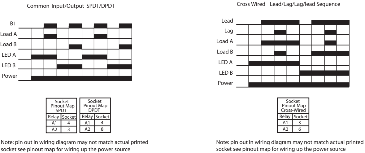
Figure 68 - Load Diagrams - 700-HTA Relays
