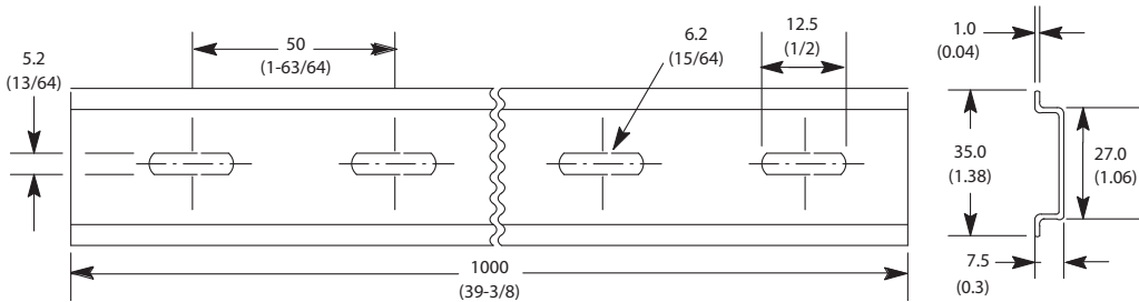
Figure 40 - Cat. No. 199-DR1 DIN Mounting Rail, Series B
