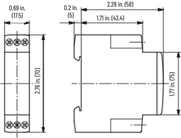
Figure 75 - Cat. No. 700-FE with 2 C/O Contacts
