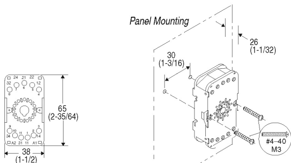
Cat. No. 700-HN101 Wire Size: 2x2.5 mm
