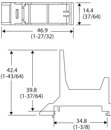
Figure 39 - Cat. No. 700-HN227
