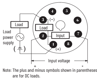
Figure 157 - Terminal Arrangement (Bottom View)
