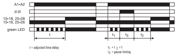
(B) OFF-delay with Auxiliary Voltage
