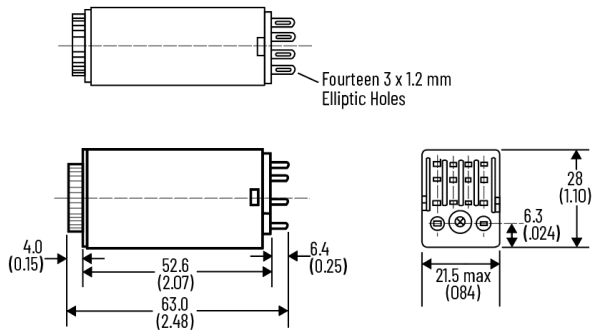
Figure 80 - Cat. No. 700-HNC
