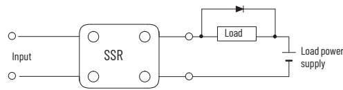
Figure 183 - DC Inductive Load Wiring
