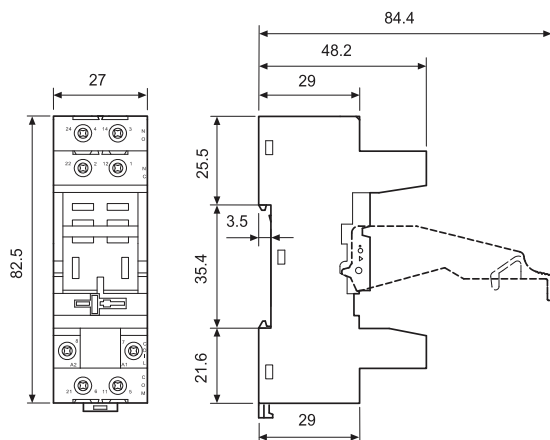
Figure 25 - Cat. No. 700-HN262
