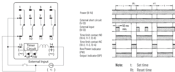
Figure 78 - Pulse Operation
