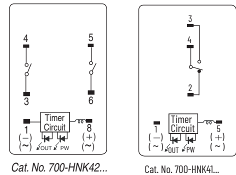
Figure 85 - Wiring
