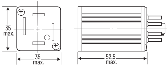
Figure 160 - Cat. No. 700-SA Relays
