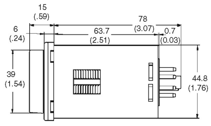
Cat. No. 700-HRY, -HRQ Timing Relays
