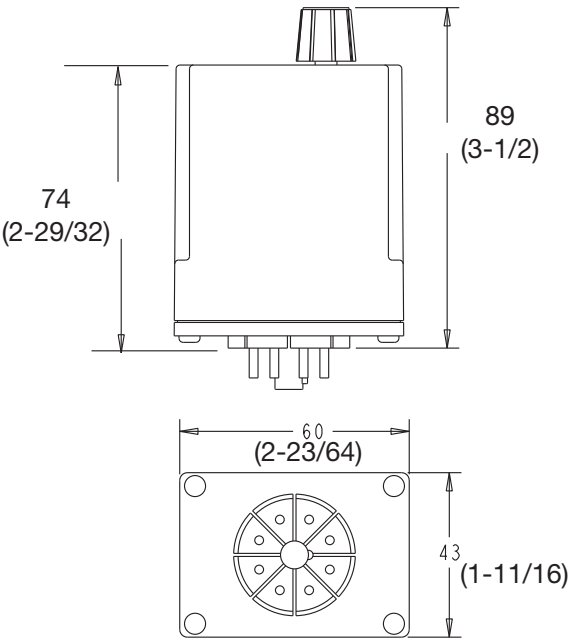
Figure 97 - 700-HT Relays
