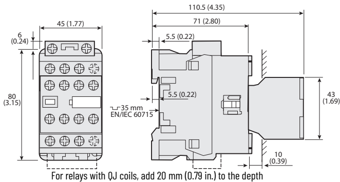
Figure 152 - 700S-EF Relays with Low-consumption Coils and Front-mounted Auxiliary Contact
