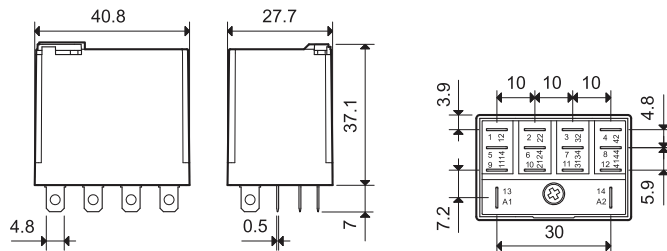
Figure 23 - Cat. No. 700-HF Relay (4PDT)
