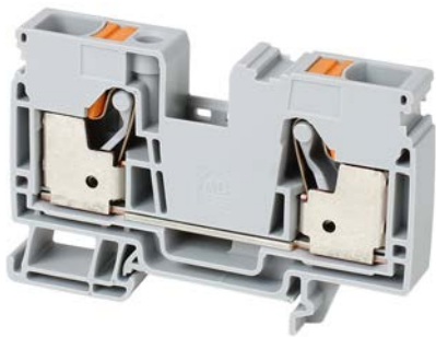
Terminal Blocks—Dimensions (W x H x L): 12 x 51.5 x 80.5 mm
