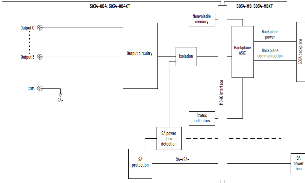
Figure 19. 5034-0B4 and 5034-0B4XT Functional Block Diagram
