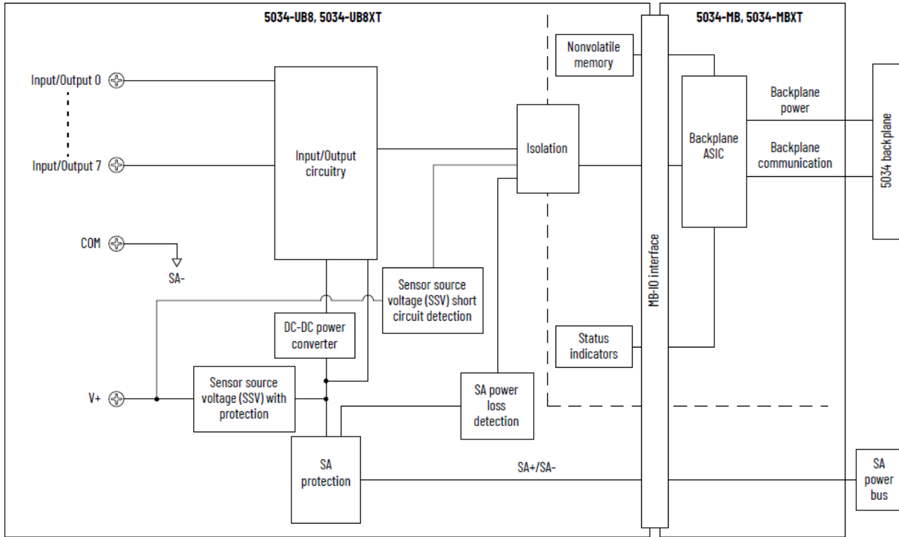
Figure 24. 5034-UB8 and 5034-UB8XT Functional Block Diagram
