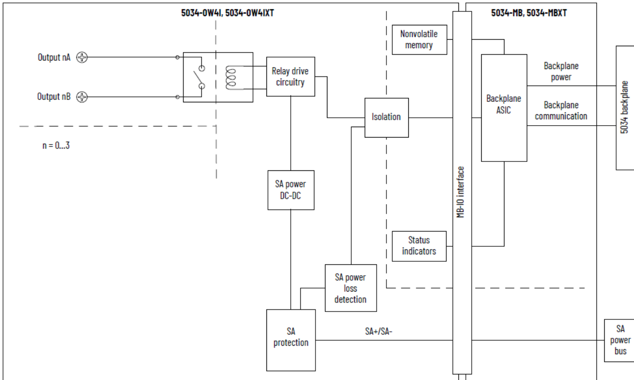
Figure 21. 5034-0W4I and 5034-0W4IXT Functional Block Diagram
