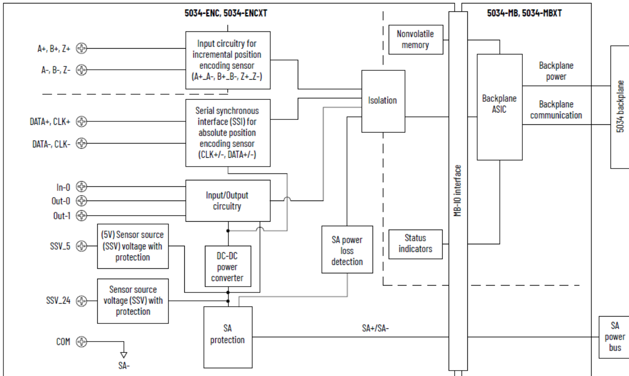
Figure 63. 5034-ENC and 5034-ENCXT Functional Block Diagram
