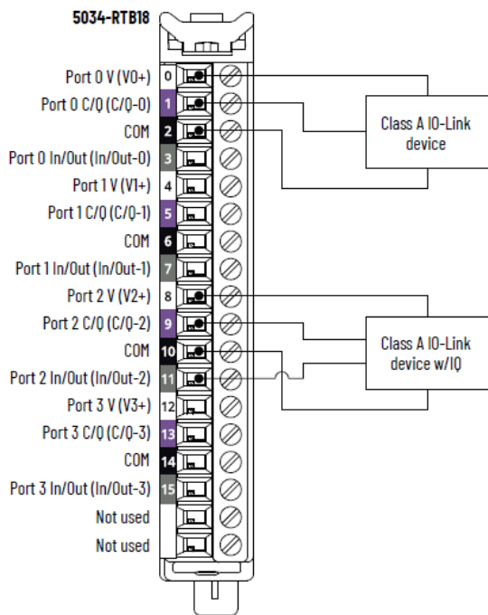
Figure 51. 5034-IOL4 and 5034-IOL4XT Wiring Diagram - IO-Link Mode
