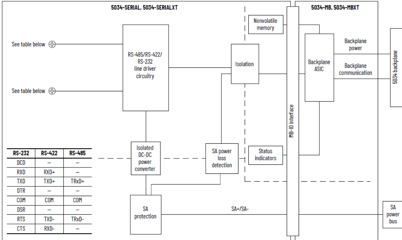
Figure 59. 5034-SERIAL and 5034-SERIALXT Functional Block Diagram
