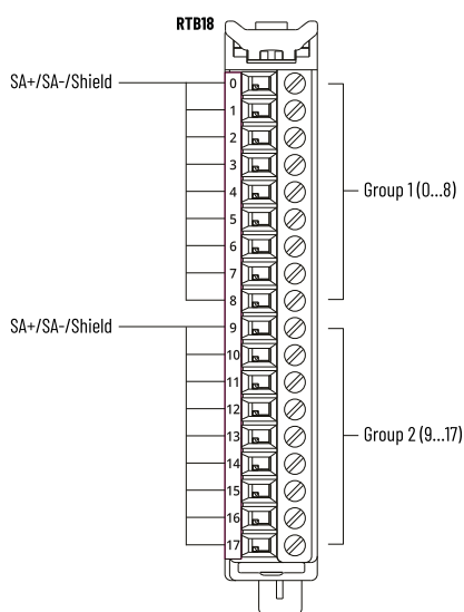
Figure 65. 5034-MBPTM and 5034-MBPTMXT Wiring Diagram
