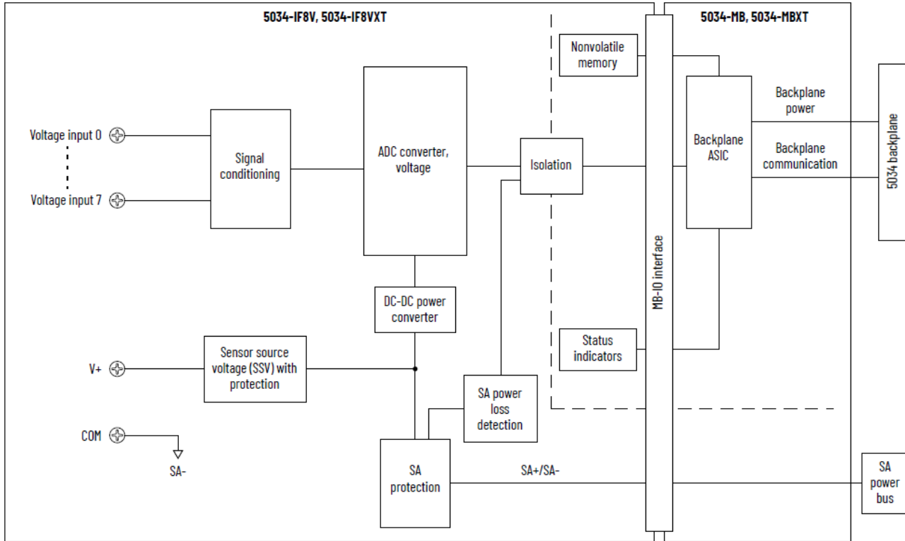
Figure 35. 5034-IF8V and 5034-IF8VXT Functional Block Diagram
