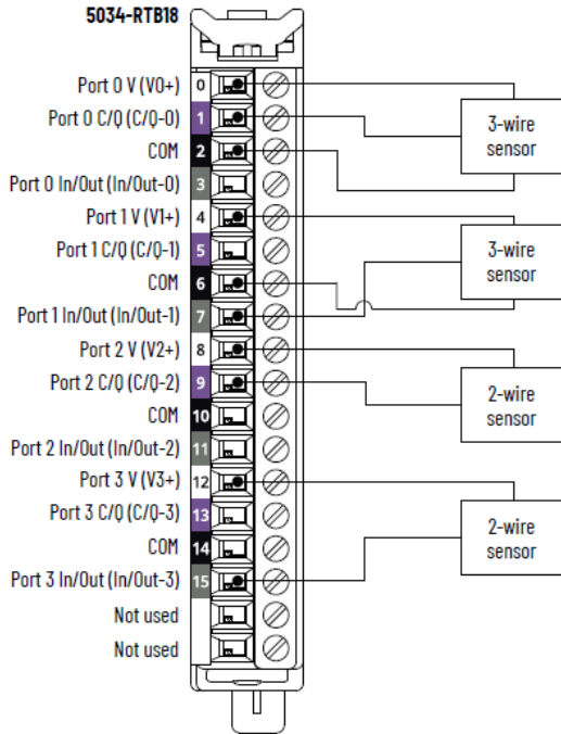
Figure 52. 5034-IOL4 and 5034-IOL4XT Wiring Diagram – DI Mode
