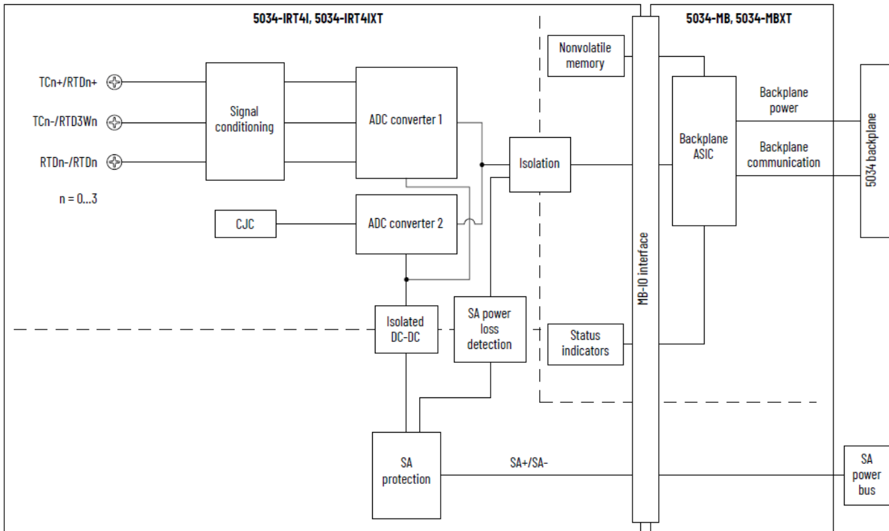
Figure 44. 5034-IRT4I and 5034-IRT4IXT Functional Block Diagram
