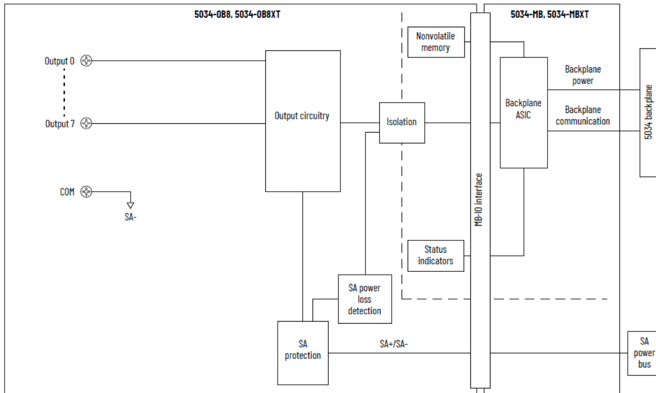
Figure 17. 5034-OB8 and 5034-OB8XT Functional Block Diagram
