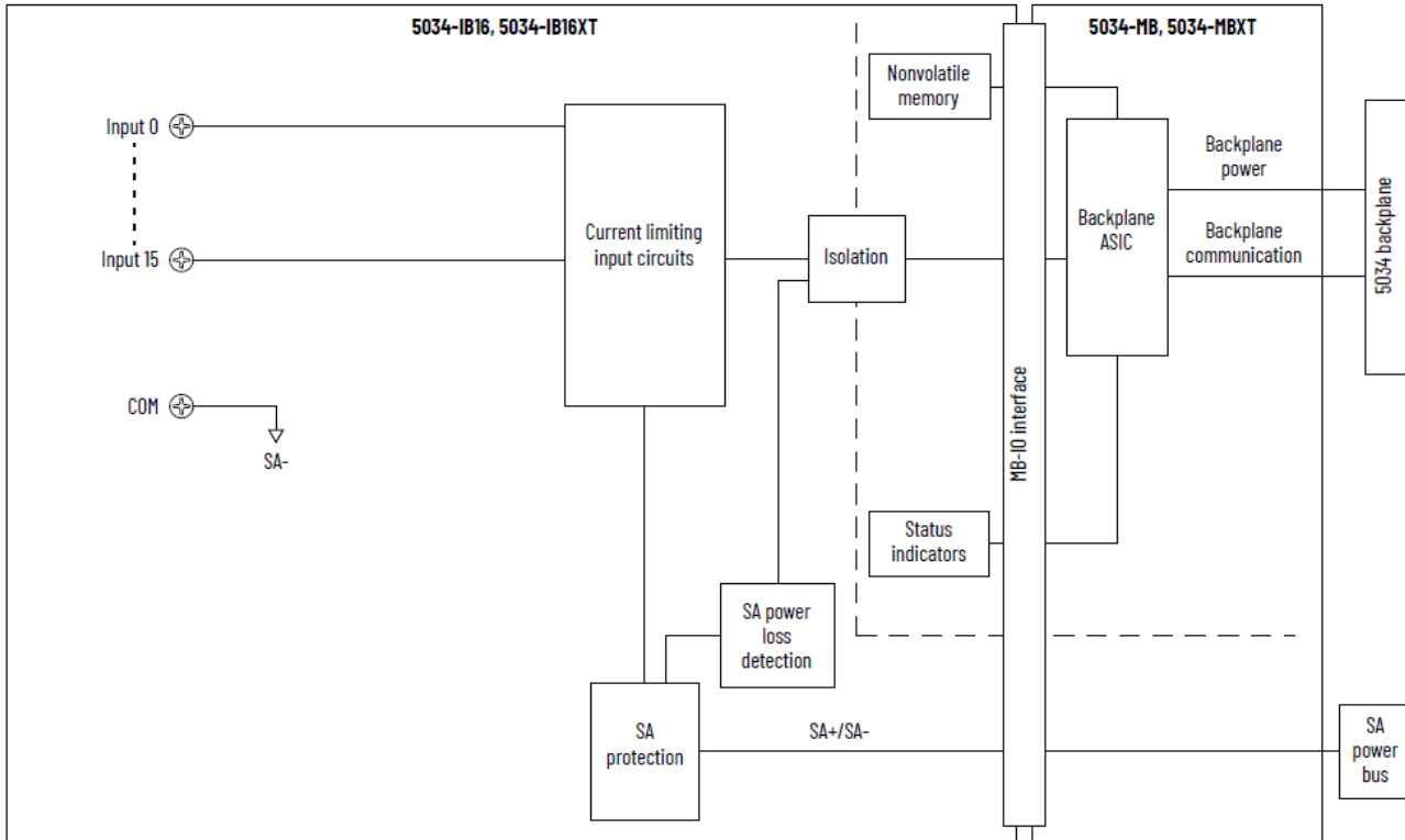
Figure 9. 5034-IB16 and 5034-IB16XT Functional Block Diagram
