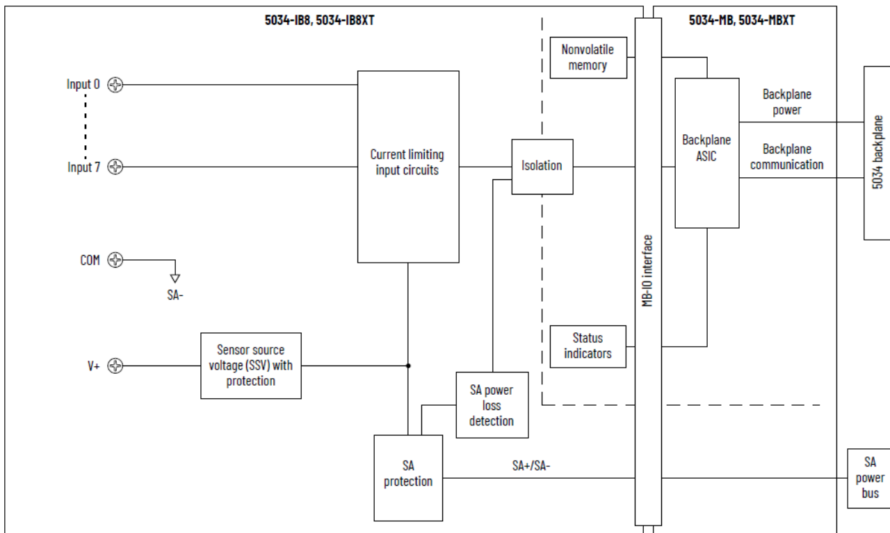
Figure 11. 5034-IB8 and 5034-IB8XT Functional Block Diagram
