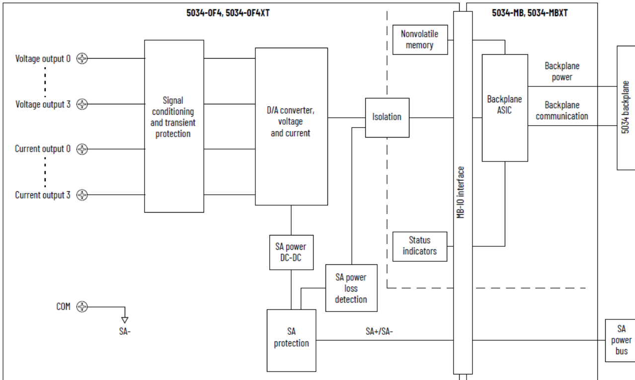
Figure 47. 5034-OF4 and 5034-OF4XT Functional Block Diagram
