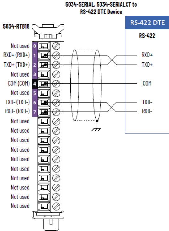
Figure 58. 5034-SERIAL and 5034-SERIALXT Wiring Diagram – RS-422 Mode
