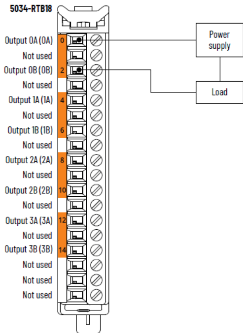
Figure 20. 5034-0W4I and 5034-0W4IXT Wiring Diagram
