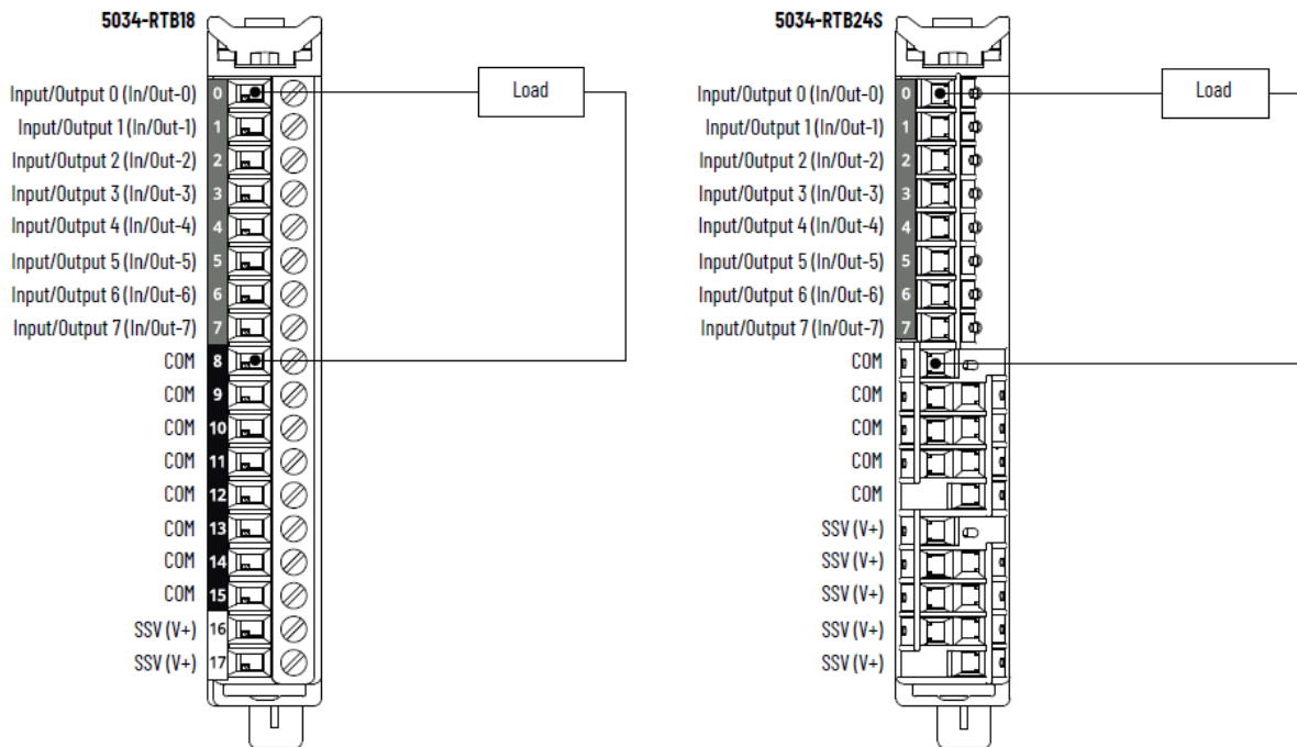
Figure 25. 5034-UB8F and 5034-UB8FXT Wiring Diagram - Output Mode
