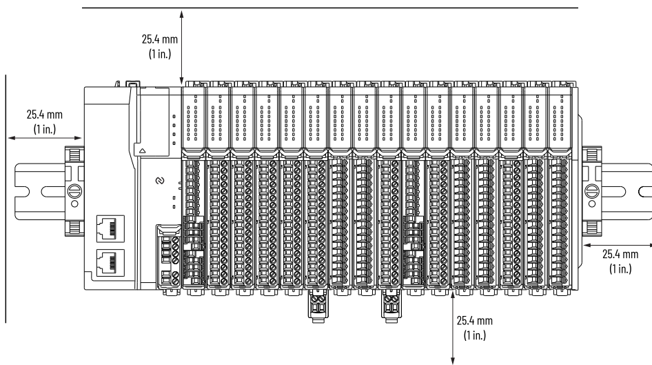
Figure 3. Spacing Example
