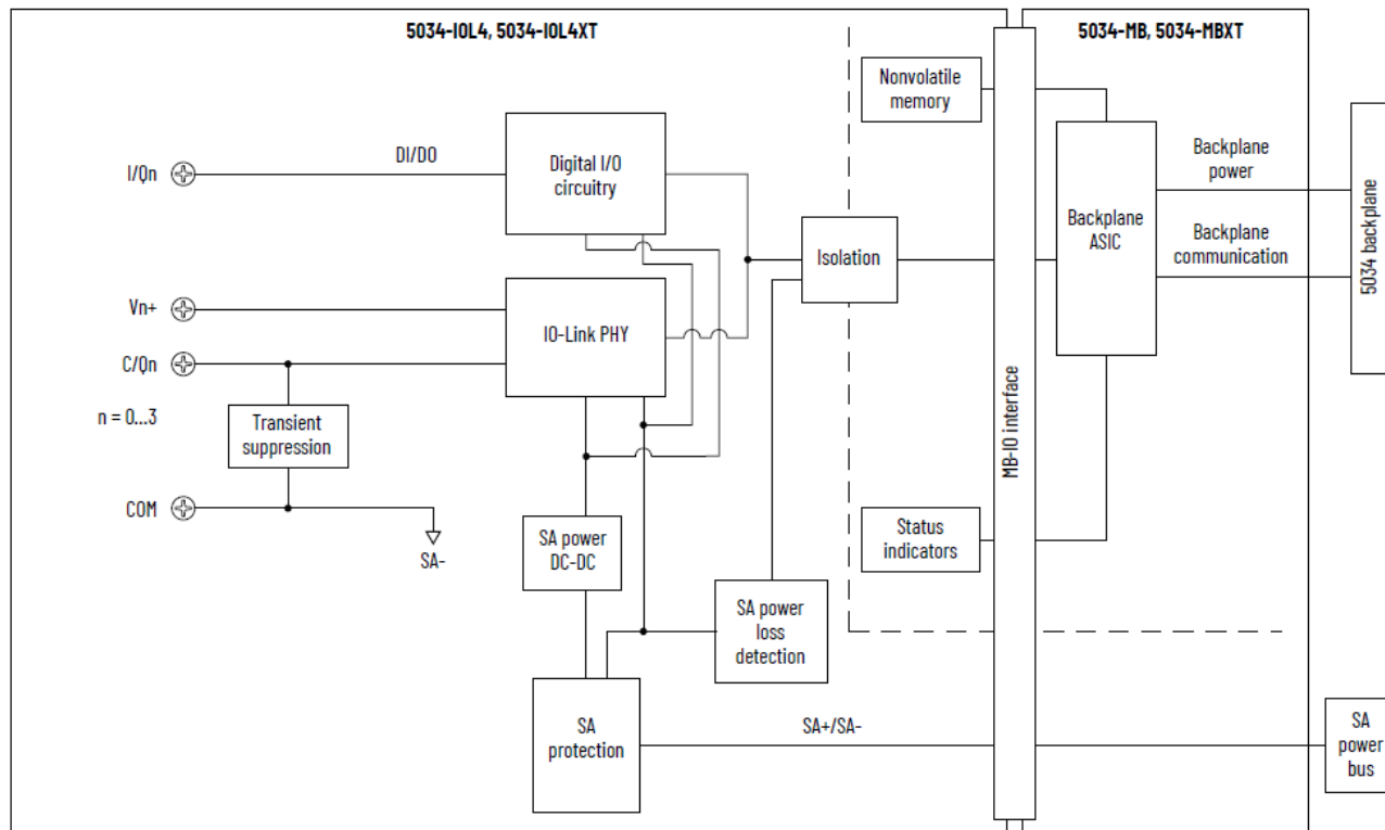
Figure 54. 5034-IOL4 and 5034-IOL4XT Functional Block Diagram
