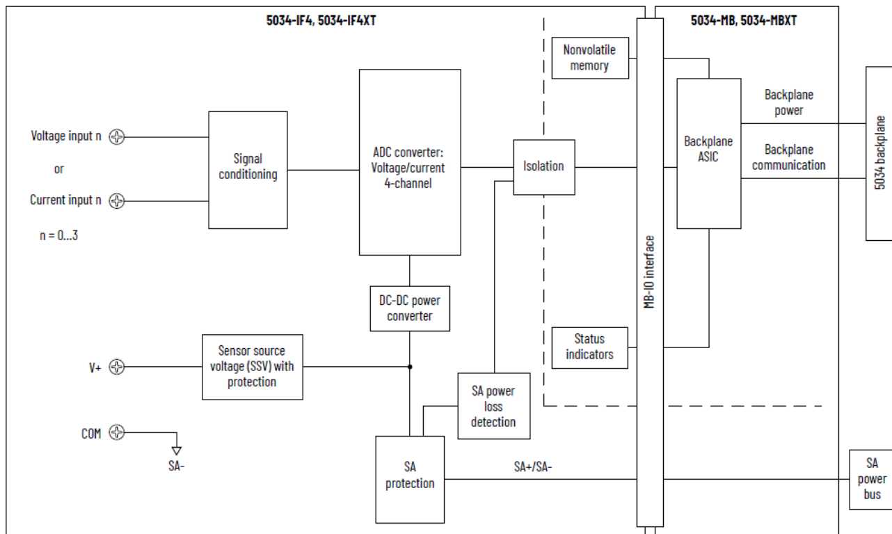
Figure 38. 5034-IF4 and 5034-IF4XT Functional Block Diagram
