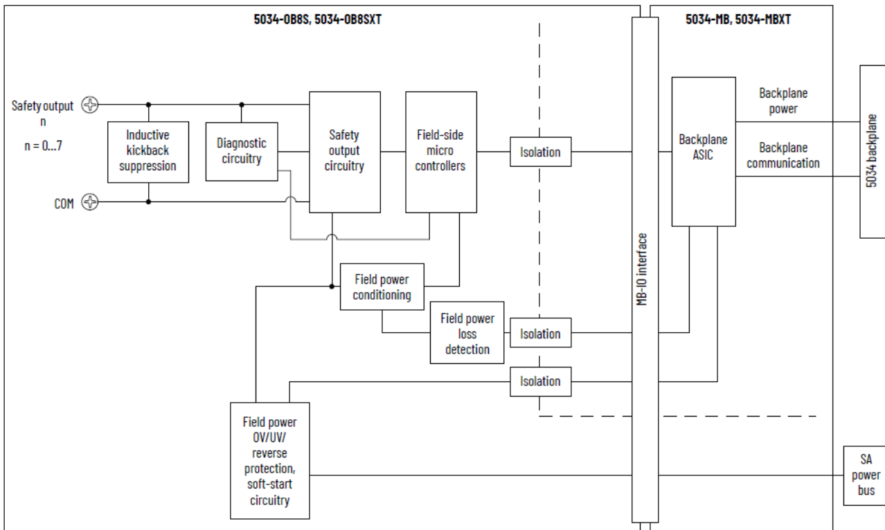
Figure 31. 5034-OB8S and 5034-OB8SXT Functional Block Diagram
