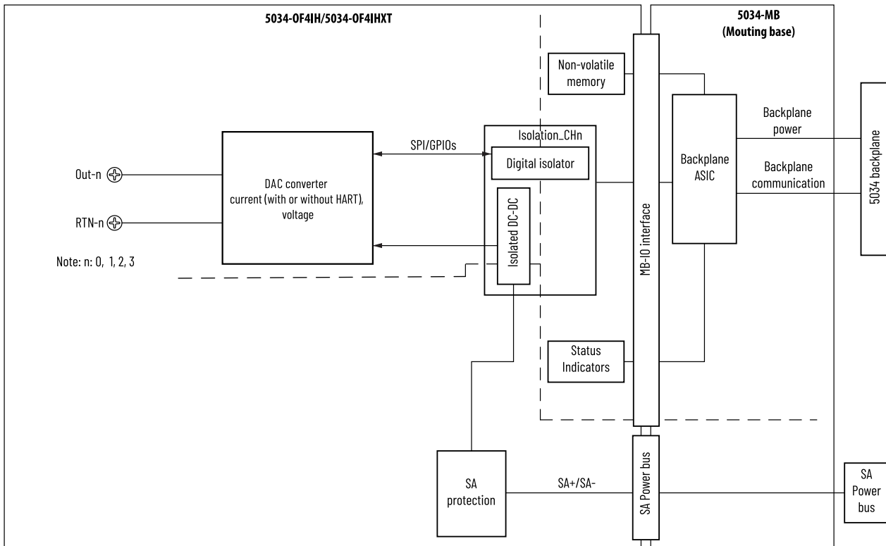
Figure 50. 5034-0F4IH and 5034-0F4IHXT Functional Block Diagram
