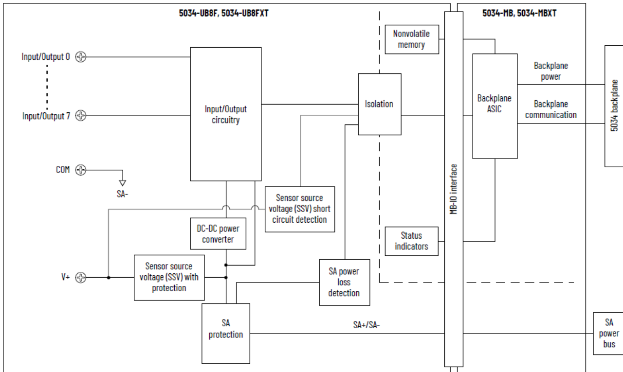
Figure 27. 5034-UB8F and 5034-UB8FXT Functional Block Diagram
