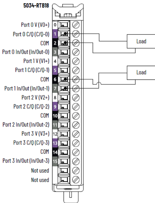
Figure 53. 5034-IOL4 and 5034-IOL4XT Wiring Diagram – DO Mode
