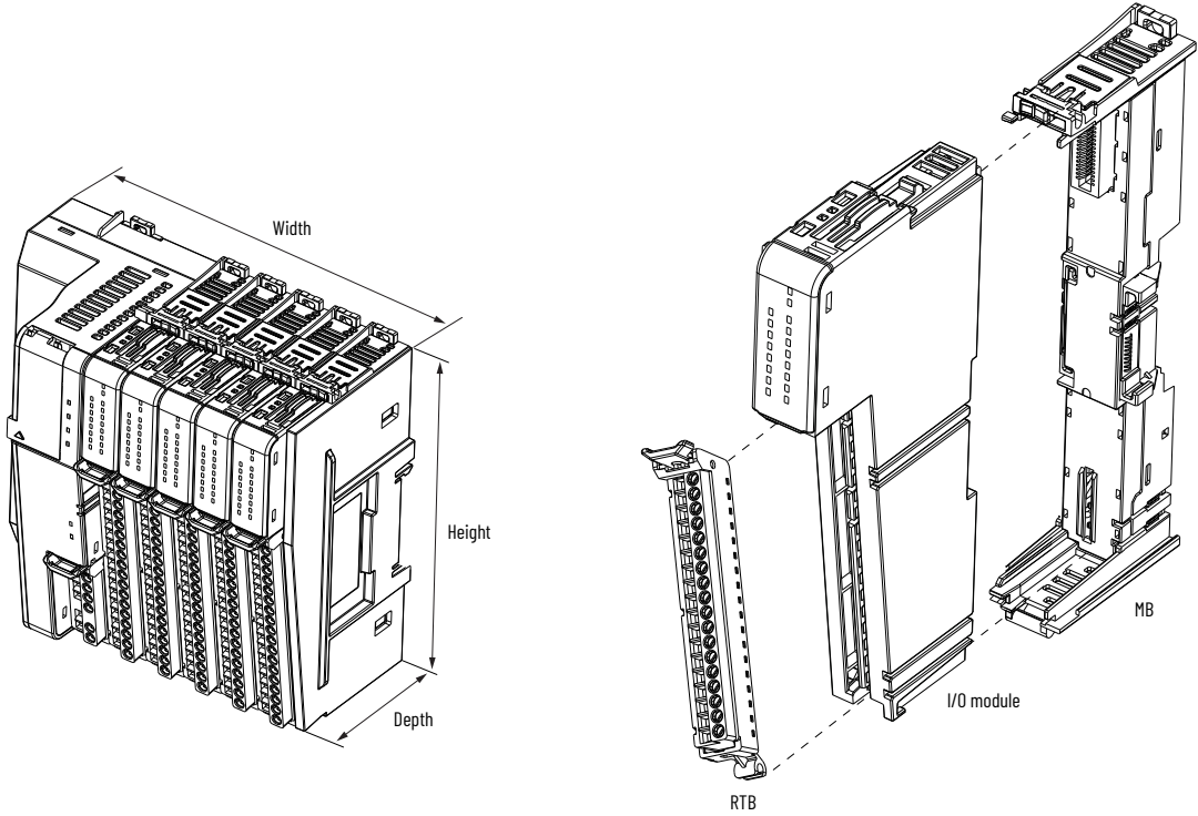
Figure 4. Dimension Example
