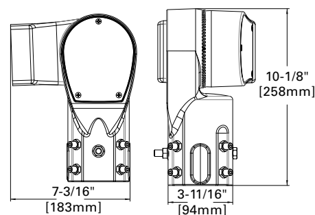
SP2=Adjustable Slipfitter 2-3/8\" (USSL-M)
