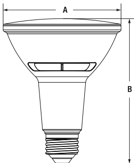
PAR30LN
