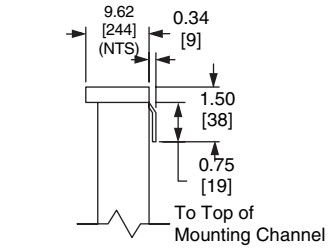
Mounting Channel Detail
