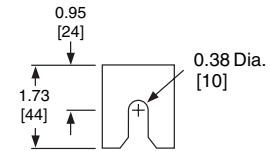
Mounting Feet
