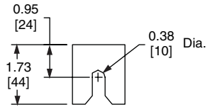
Mounting Foot
