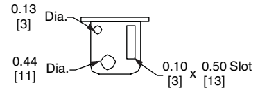
Seal Bracket
