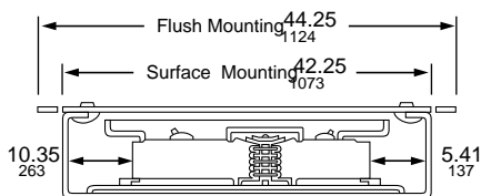
Typical Mounting of BD, BG, BJ, BK, HD, HG, HJ, HL, JD, JG, JJ, JL, LA, LD, LJ, LL, LR, MG, MJ, PG, PJ, PK, PL, QB, QD, QG, QJ Circuit Breakers
