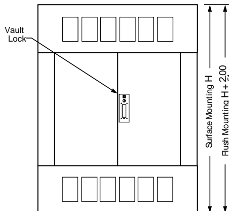
Typical 4-Piece Trim with Optional Door
