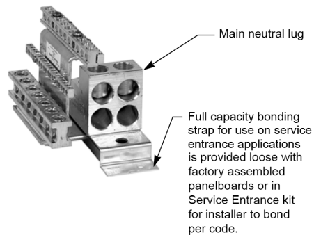
Typical Solid Neutral
