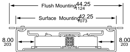
Typical Mounting of BD, BG, BJ, BK, HD, HG, HJ, HL, JD, JG, JJ, JL, LA, LJ, LL, LR, MG, MJ, PG, PJ, PK, PL, QB, QD, QG, QJ Circuit Breakers
