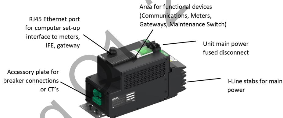
Typical Layout for I-Line Enable module (U-PaS for Wide Side Left shown)
