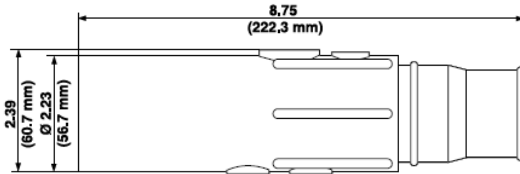
Male Plug - Double Set Screw Detachable
