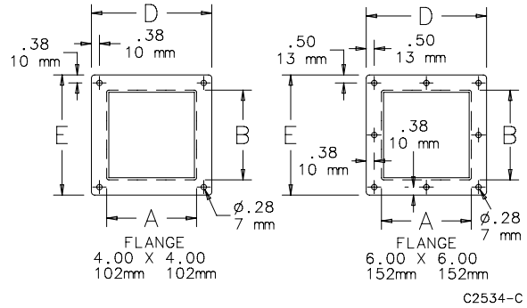
Flange Detail
