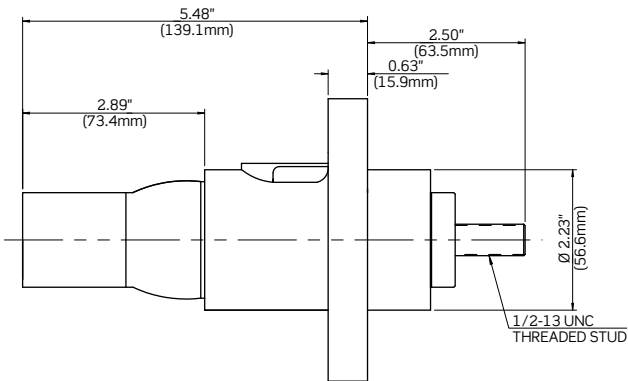
Side View 90° Female Panel Receptacle, Threaded Stud
