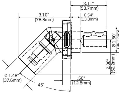
Typical for Double Set Screw Termination
