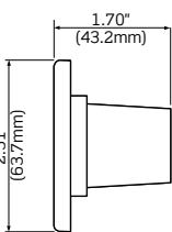
Male Protective Cap
