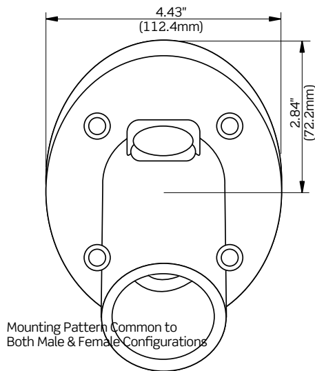
Front View 30° Panel Receptacle
